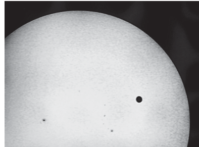
Figure 14. Venus Transit and Sunspots.
