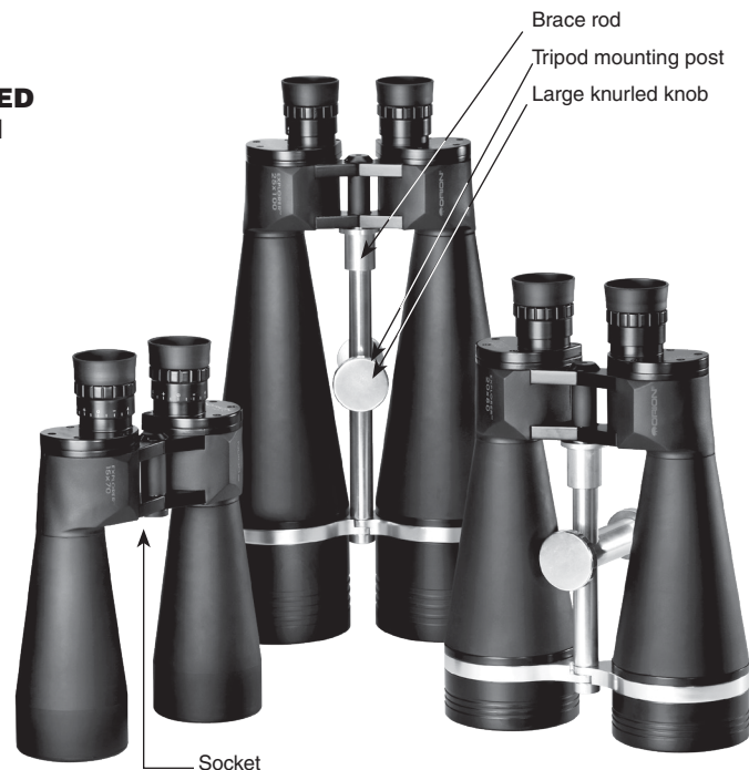
Figure 1. The GiantView 70mm, 80mm, and 100mm binoculars. Not shown: 16x80 ED, 20x80 ED, 20x100 ED.
